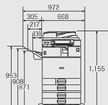
Sestava SR3130 PB3160
