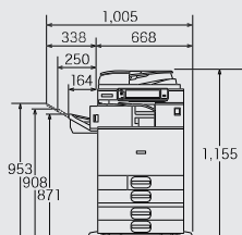
Sestava SR3130 + PU3040 PB3160
